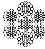
6x31 Seale
